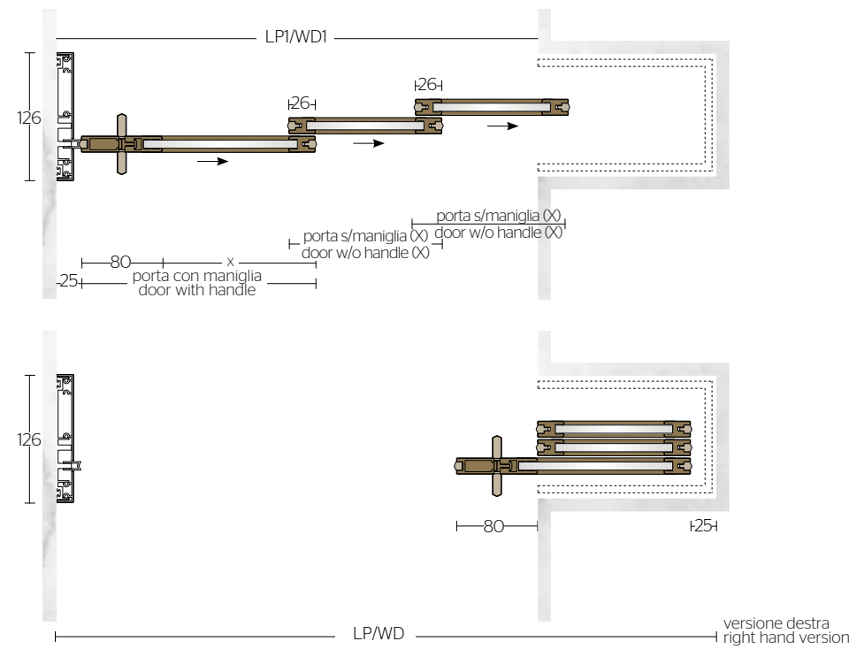
3 SLIDING DOORS WITH RECESSED COMPARTMENT SCORREVOLI A 3 PORTE CON VANI AD INCASSO
