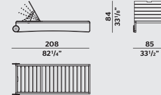
SUNBED TEAK VERSION LETTINO VERSIONE TEAK
