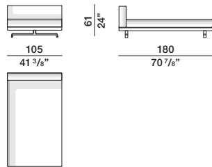
corner island element IA224A dx - sx
