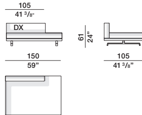
island element IS150A dx - sx
